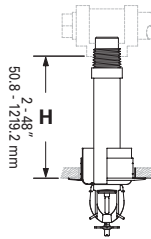
Type 1 Flush Escutcheon Flush Rosette Rosace standard
